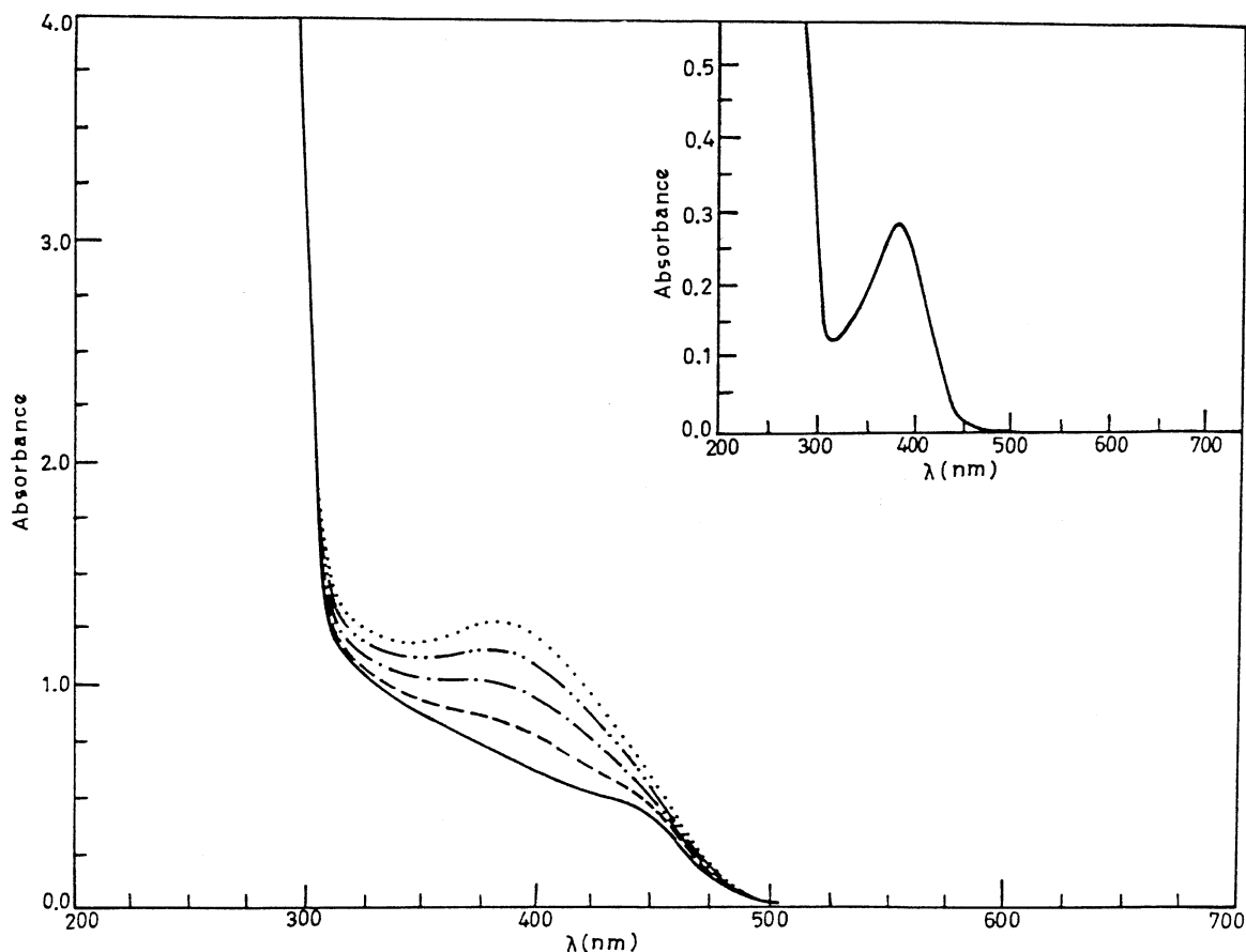
Figure 1. Electronic spectra of the reaction mixture containing 0.4 mM colloidal CdS and 4.0 mM 2-MI as a function of irradiation time: (—)0; (---)2; (- · -)5; (- · · -)10; (...)15 min. Inset: electronic spectrum of the chloroform extract of the product.
