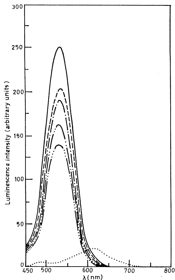
Figure 3. Luminescence spectra of 0.24 mM colloidal CdS in the absence (...) and presence of various concentrations of 2-MI: (---)0.5; (-.-)1.0; (-.)1.5; (—)2.0; (—)2.5 mM.
