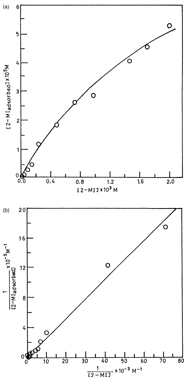
Figure 2. (a) Adsorption isotherm of 2-MI on colloidal CdS. (b) Plot of Langmuir adsorption isotherm of 2-MI.
